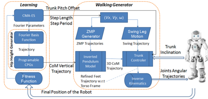
Fig 3. The interaction between each component of the proposed approach
